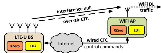
Figure 1: LTE-U BS with Xzero performs CTIN towards co-located WiFi nodes.
